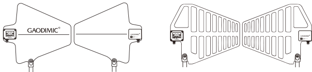
ANT241P-D1/D2 Active Directional Antenna (2026)
