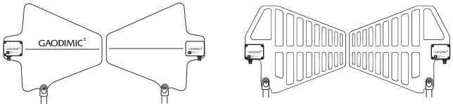
ANT241P-DP1/DP2 Passive Directional Antenna (2026)
